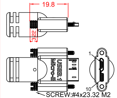
CBL-HFD3SAB6MBH-Xm with short locking screws
